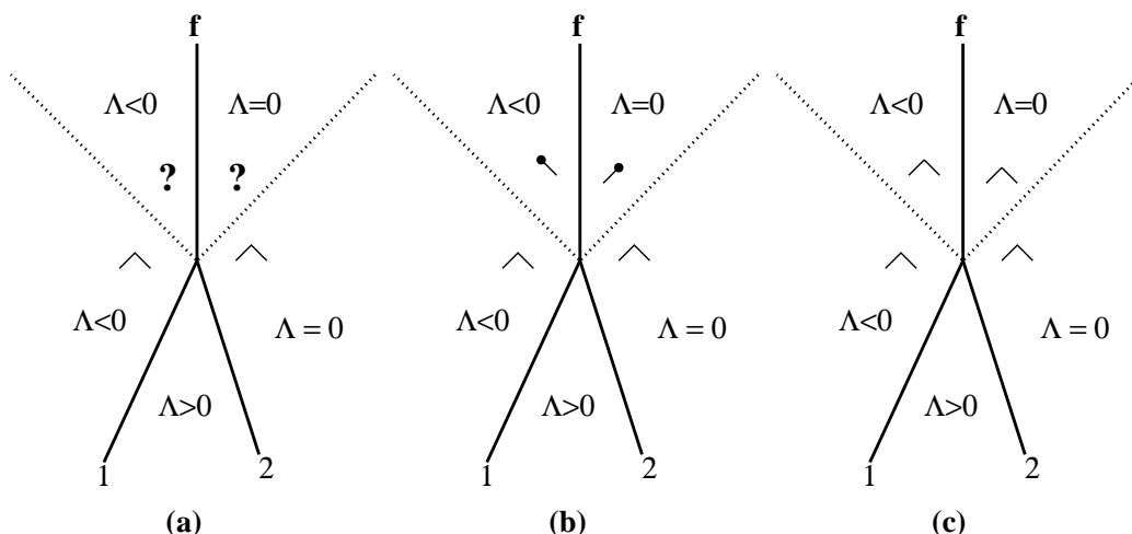
Figure 11: This figure demonstrates how to determine the direction of the Bousso wedge in the spacetime to the future of the collision, when the collision happens at a radius R < \ell . Outside the future lightcone of the collision, the wedges have the behavior shown in figure 10. Inside the future lightcone, we do not know the direction yet, as shown in (a). Continuity of R across the null shell partly determines the behavior inside the future lightcone, as shown in (b). Here the dots denote the vertex of the wedge. Now imagine starting in the \Lambda = 0 region and following the known decreasing null ray across the final domain wall. This ray is left-moving and past-directed. R must continue to decrease along this ray after crossing the domain wall since we have assumed the null energy condition, so in the \Lambda < 0 region the left-moving past-directed ray must decrease. We can repeat the same argument reversing the two sides of the domain wall, leading to the final diagram (c).
