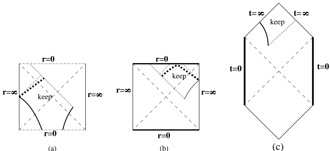
Figure 6: The full diagram, figure 5, is constructed from the pieces shown here. In the thin wall approximation, (a) is the conformal diagram for AdS spacetime in H_2 slicing. The top and bottom dot-dashed lines are coordinate singularities where the size of the H_2 goes to zero. The region we use, labelled “keep” in the figure, is bounded by the domain wall (heavy curved lines) and the shell of radiation emitted from the collision (dotted line). As described in the text, the thin wall solution has a Cauchy horizon (thin, short dashes). Going beyond the thin wall approximation, the Cauchy horizon will be removed by a spacelike curvature singularity (heavy dashed line). Diagram (b) is the hyperbolic AdS black hole. The region we use is bounded by the null shell of radiation and the domain wall. The curvature singularity of (a) must continue across the null shell into (b). Just as in (a), a Cauchy horizon forms at the point where the domain wall hits the boundary, so again a curvature singularity must cut off the boundary at the point where the domain wall hits it. Diagram (c) is the hyperbolic \Lambda = 0 solution, bounded by the domain wall and the null shell radiated into the \Lambda = 0 side of the domain wall. Note that we do not use the part of the spacetime which contains timelike singularities.
