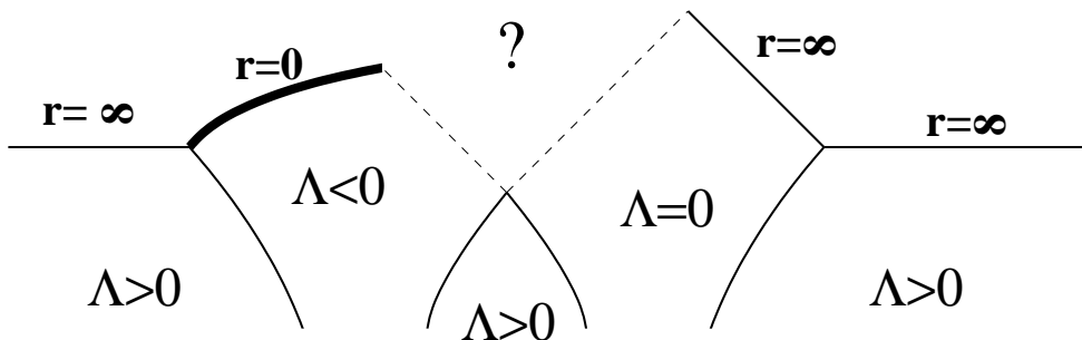
Figure 1: Bubbles with zero and negative cosmological constant can collide. The heavy black line denotes the curvature singularity which always forms in the \Lambda < 0 bubble. The \Lambda = 0 bubble always includes a piece of future null infinity. We will investigate what happens to the future of the collision.
