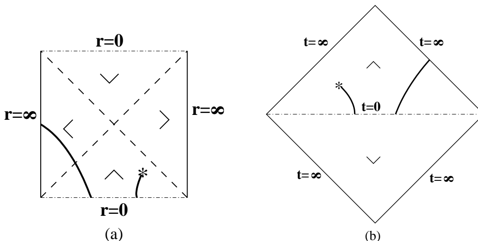
Figure 10: “Bousso wedges” indicate in which null directions the curvature radius of the hyperboloids decreases. Figure (a) is a piece of AdS spacetime, while (b) is a piece of Minkowski spacetime. The collision occurs at the point marked with a star(*). When the collision occurs at R < \ell , it is “behind the horizon” in AdS, as shown in (a).
