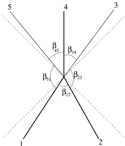
Figure 12: The absence of a conical deficit at the collision point leads to a constraint on the relative boosts \beta of the colliding domain walls, equation (A.3).
