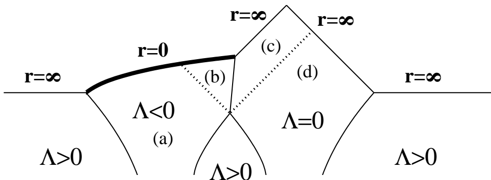
Figure 5: A sketch of the conformal diagram for a collision in which the resulting domain wall has tension exceeding the BPS bound. In the thin wall approximation, region (a) is a piece of AdS spacetime, (b) is a piece of the hyperbolic AdS black hole, (c) is a piece of the hyperbolic Schwarzschild solution, while (d) is a piece of Minkowski spacetime. Going infinitesimally beyond the thin wall approximation results in additional singularities to create a diagram like the one shown here. In the next figure, we show the regions (a), (b), and (c) in more detail.
