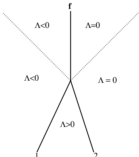
Figure 3: In our thin wall approximation, the spacetime near the collision is divided into five regions. The dotted lines denote outgoing shells of radiation. The solid lines denote two incoming bubble walls and the outgoing domain wall.
