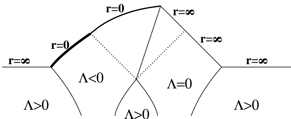
Figure 7: If the tension saturates the BPS bound, the domain wall reaches infinity in infinite time outside the AdS-Schwarzschild black hole.
