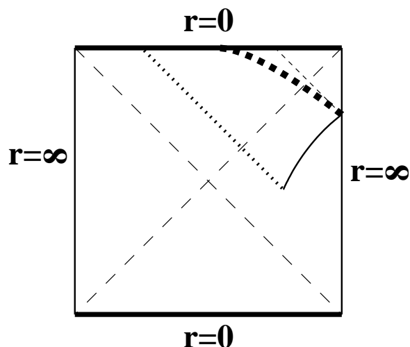
Figure 4: If \kappa \neq 1/\ell , the domain wall accelerates out to infinity in finite time in the AdS-Schwarzschild black hole. As we explain later, we expect a singularity to form along the heavy dashed line.
