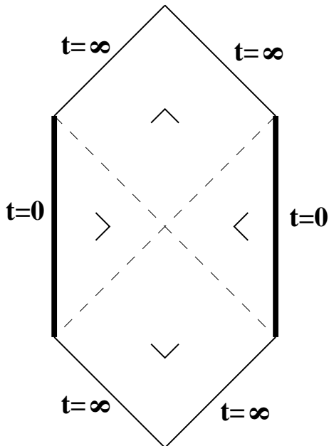
Figure 2: The Penrose diagram for the “hyperbolic Schwarzschild” spacetime. Each point represents a hyperboloid and the singularities are timelike. We will only be interested in the region to the future of the surface t = t_0 (denoted by the dashed line), so these singularities will not enter our discussion. The “wedges” will be explained in section 2.5.
