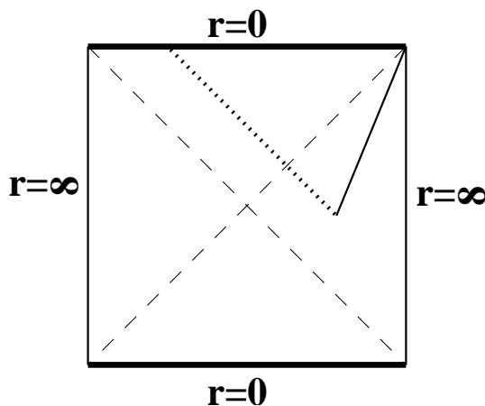
Figure 7: If the tension saturates the BPS bound, the domain wall reaches infinity in infinite time outside the AdS-Schwarzschild black hole.
