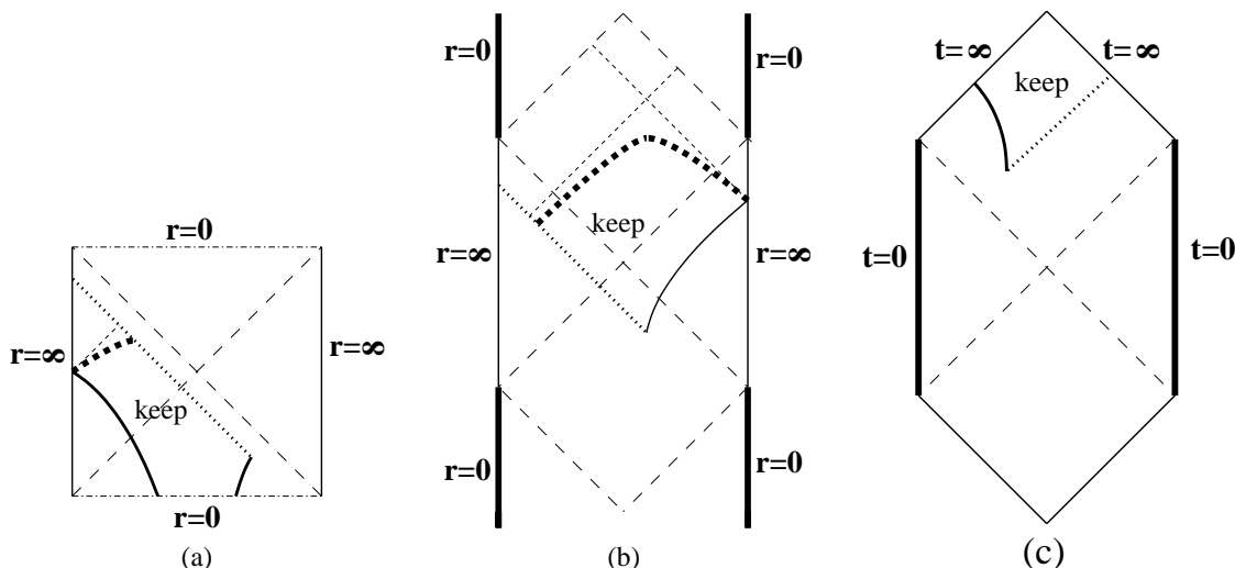
Figure 9: In the case that the collision occurs on an H_2 with radius of curvature less than the AdS scale, the situation is slightly different from figure 6. In this case, the null shell of radiation on the \Lambda < 0 side of the domain wall ends up behind the white hole horizon. Also (b) is now a hyperbolic AdS black hole with negative M .
